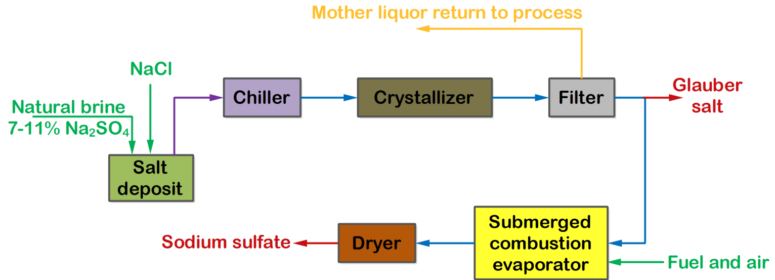
Figure: Manufacture of Sodium sulfate from natural brine
